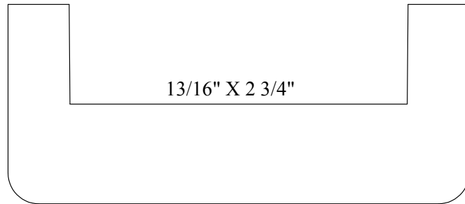
SHOERAIL 9369 1 5/8" X 3 3/4"
