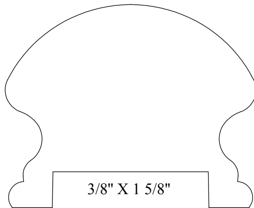
HANDRAIL 92633 2 1/8" X 2 5/8"
