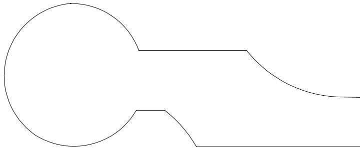
HANDRAIL 93755 1 1/2" X 3 3/4"
