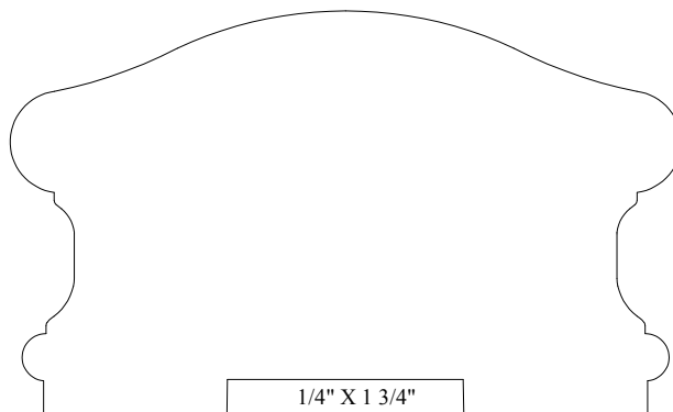
HANDRAIL 950015 3" X 5"
