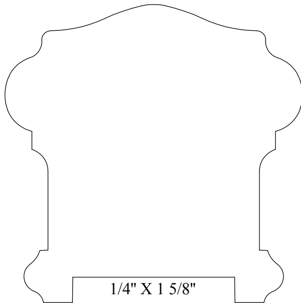
HANDRAIL 930017 3" x 3"
