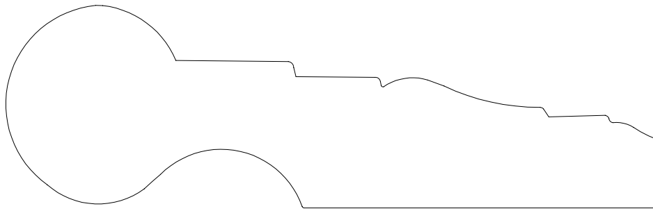
HANDRAIL 9494 1 1/2" X 4 7/8"
