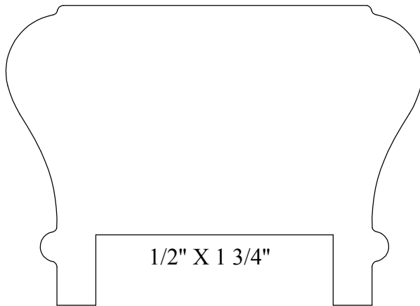
HANDRAIL 9313 2 1/4" X 3 1/8"
