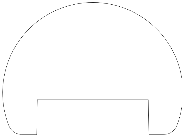
HANDRAIL 932515 2 3/8" X 3 1/4" ( 5/8" X 2" PLOW)
