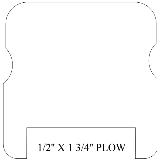
HANDRAIL 250 2 1/2" X 2 1/2"
