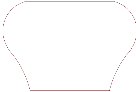
HANDRAIL 922513 1 17/32" X 2 9/32"
