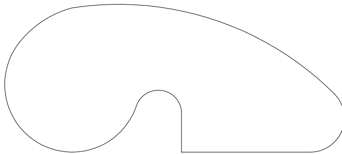
HANDRAIL 935033 1 1/2" X 3 1/2"
