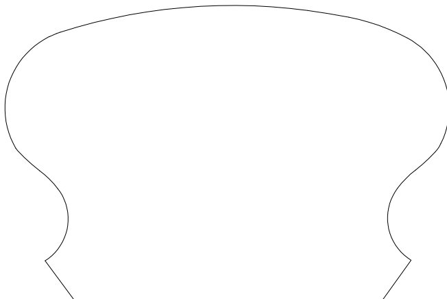
HANDRAIL 942510 2 7/8" X 4 5/16"
